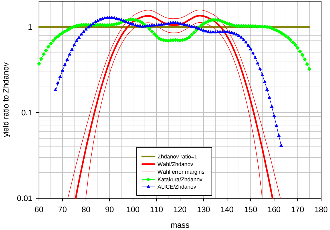
Benchmark B: ^{241}\text{Am} at 50 MeV, post neutron emission yield ratios to Zhdanov's data
